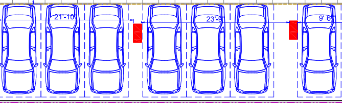
GROUND FLOOR PLAN (PARKING # 30 nos)
